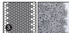
Integral B+W 031 3-Schicht-Platte \lambda_D = 0.031 W/mK 15 kg/m 3
